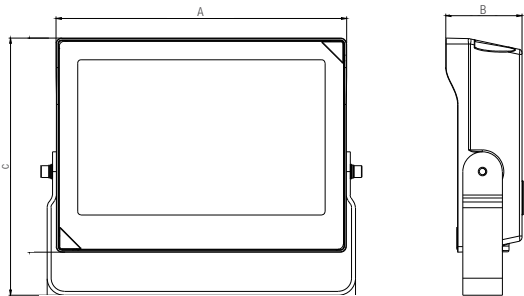
Yoke Mount
