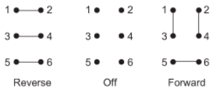
Internal Switching
