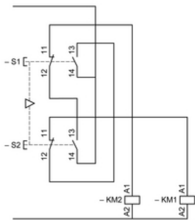
Control of Single-Speed Reversing Motor With ZBE2BE101 + ZB2BE102
