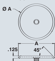
STAINLESS STEEL STUD 10-32 X 5/8"
