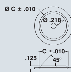
INSIDE WASHER
