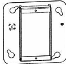
Details Part #: 52C49-1 1/2 Box Quantity: 50
