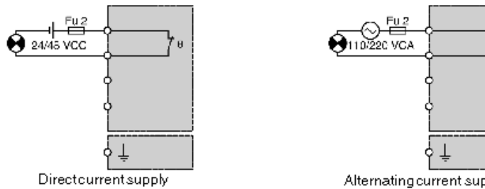
Directcurrentsupply
