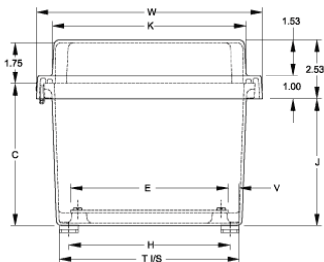
End View
