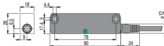
ST H••••M• sensor with M12 connector
