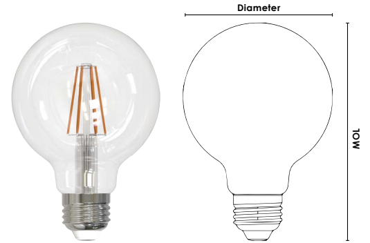
MOL : 4 5/8 in. (118 mm) Dia. : 3 1/8 in. (80 mm)
