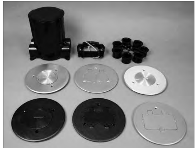
Ratchet-Pro Series Floor Box shown with available accessories and covers.
