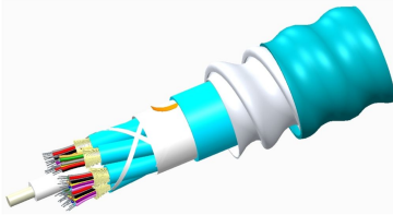
LazrSPEED® Riser Distribution Cable, interlocking aluminum armored with riser jacket, 6 fiber single-unit
