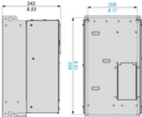
Drives Without Top Cover, Without EMC Plate
