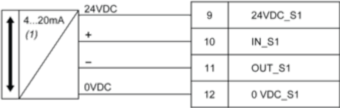
(1) : Sensor 3 Wires Voltage Sensor
