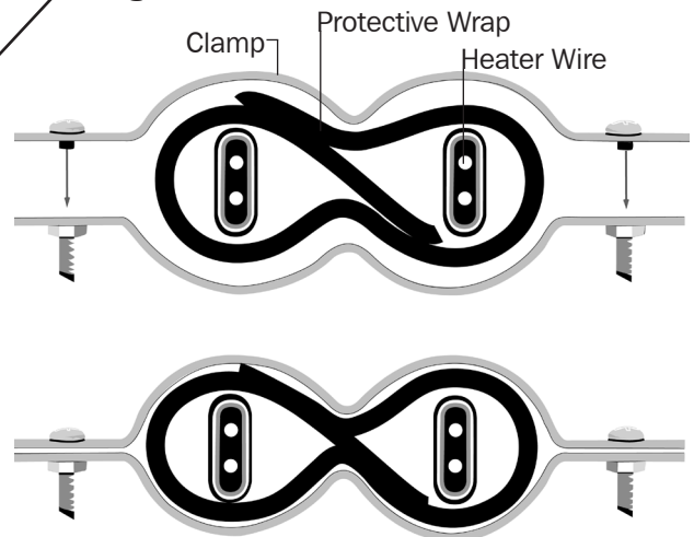
Figure 2 - Cross section view of clamp
