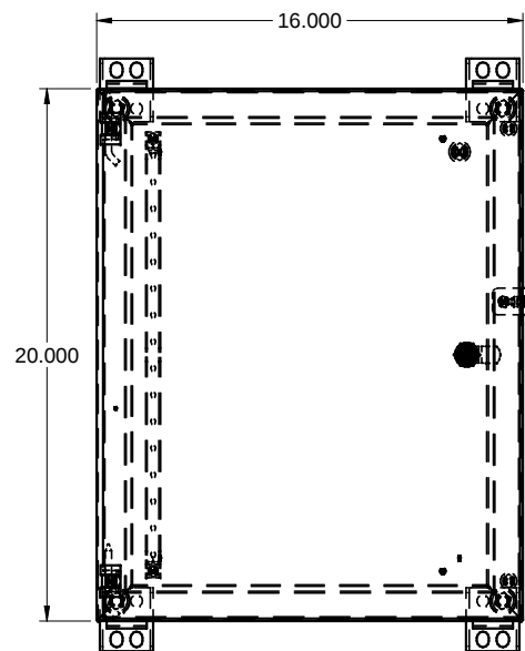
FRONT / FACE
