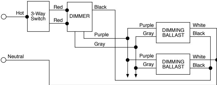
Figure 2 – 3-Way Wiring
