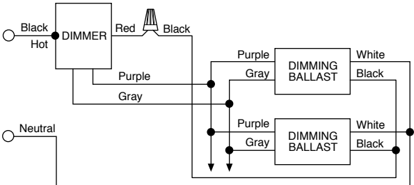
Figure 1 – Single Pole Wiring
