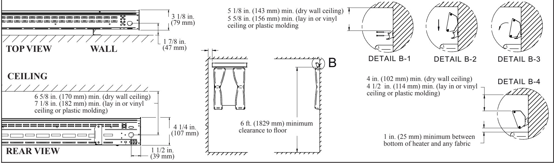
Figure 4 - MOUNTING RESTRICTIONS
