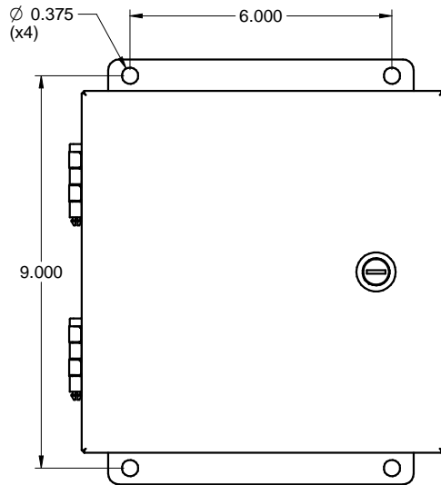
FRONT / FACE
