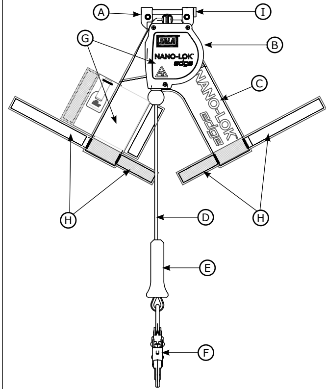
Figure 13 – SRL-LE Inspection
