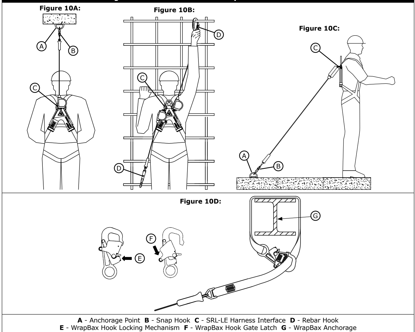
Figure 10 – Nano-Lok SRL-LE System Connections
