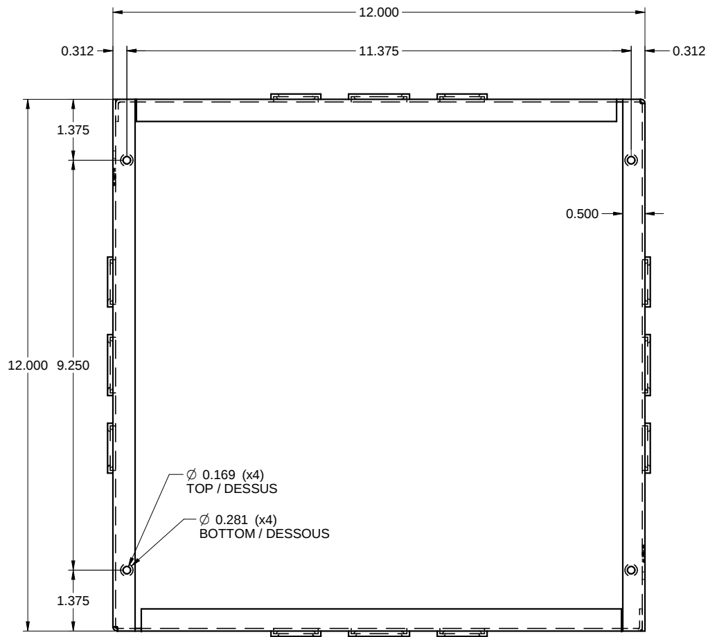
FRONT / FACE
