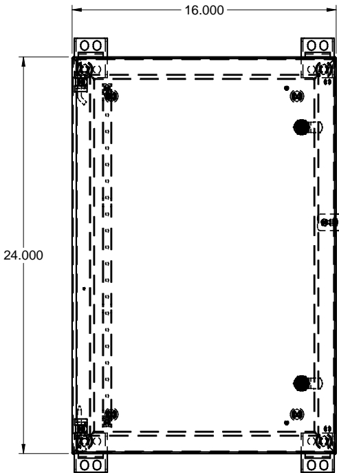
FRONT / FACE
