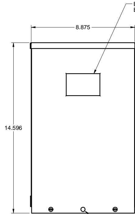
FRONT / FACE
