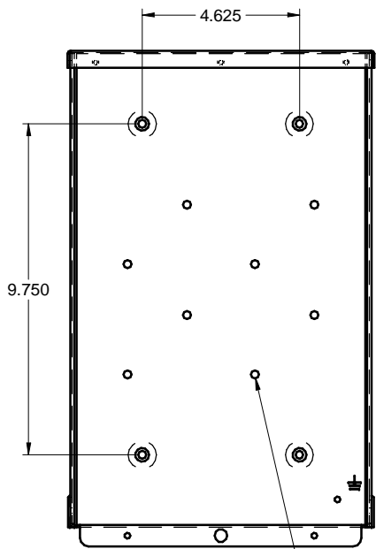
FRONT WITHOUT COVER FACE SANS COUVERCLE
