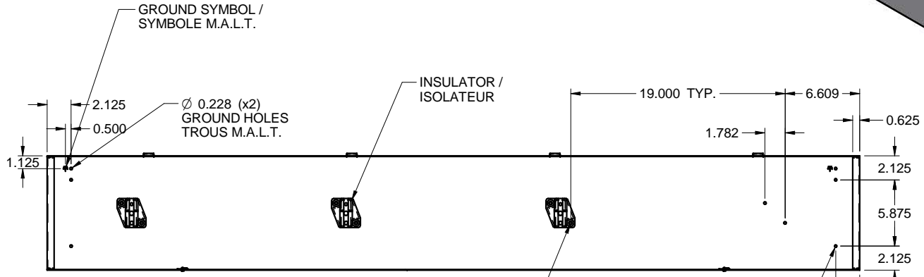
TOP WITHOUT COVER DESSUS SANS COUVERCLE
