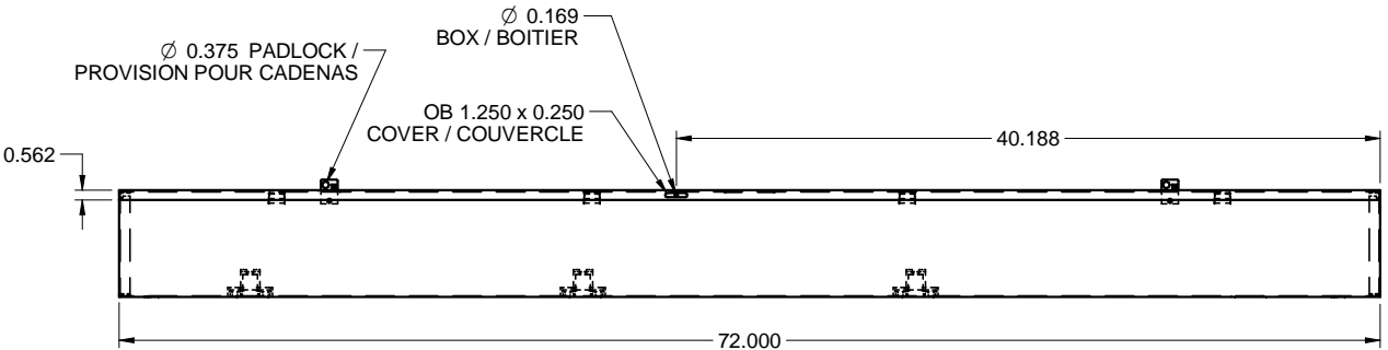
FRONT / FACE
