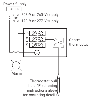
Figure 2. Low-temperature alarm
