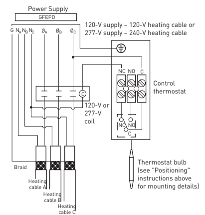
Figure 4. Contactor control
