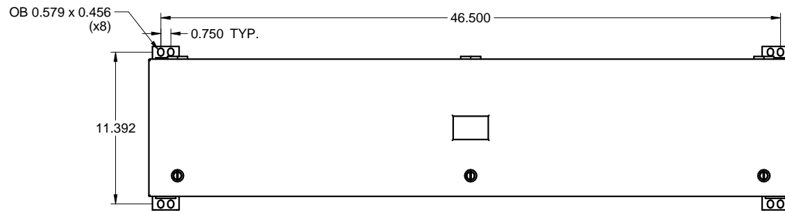
FRONT / FACE
