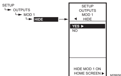
Fig. 54. Installation - Sorties - Mod 1/2 - Masquer.
