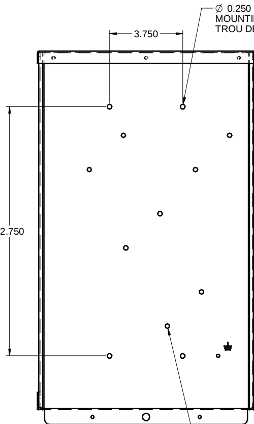
DETAIL A
