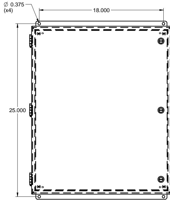
FRONT / FACE
