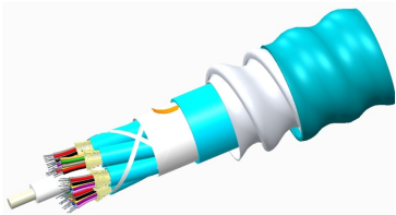
LazrSPEED® Plenum Distribution Cable, interlocking aluminum armored with plenum jacket, 12 fiber single-unit
