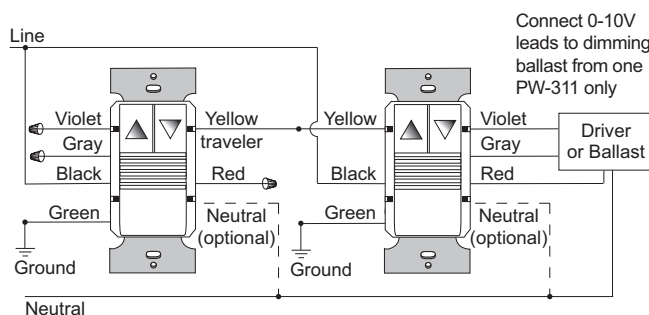
Multi-way wiring
