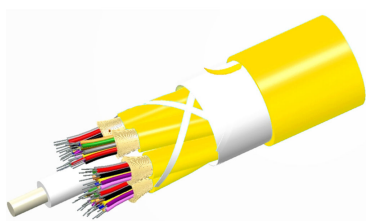
TeraSPEED® Riser Distribution Cable, 96 fiber multi-unit with 12 fiber subunits
