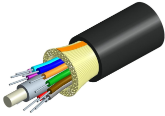
LazrSPEED® Indoor/Outdoor Plenum Distribution Cable, 6 fiber single-unit
