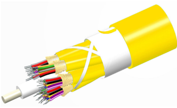
TeraSPEED® Riser Distribution Cable, 48 fiber multi-unit with 12 fiber subunits
