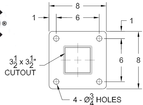
Baseplate Detail
