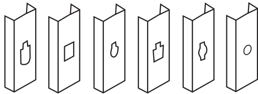
Common hole configurations in metal studs.
