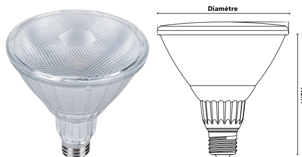
LHTM: 5" (127 mm) Dia. : 4 23/32" (120 mm)
