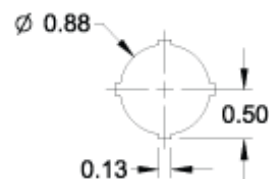
22.5mm Detail
