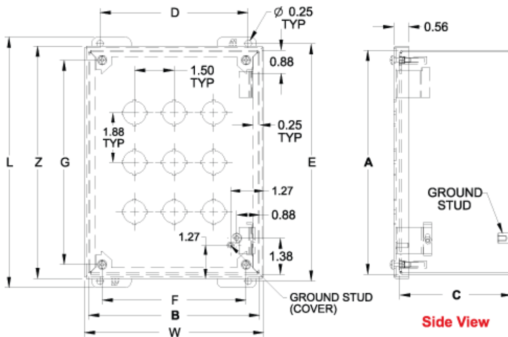
Front View Body Type MPB6 through MPB12 (Hinged)
