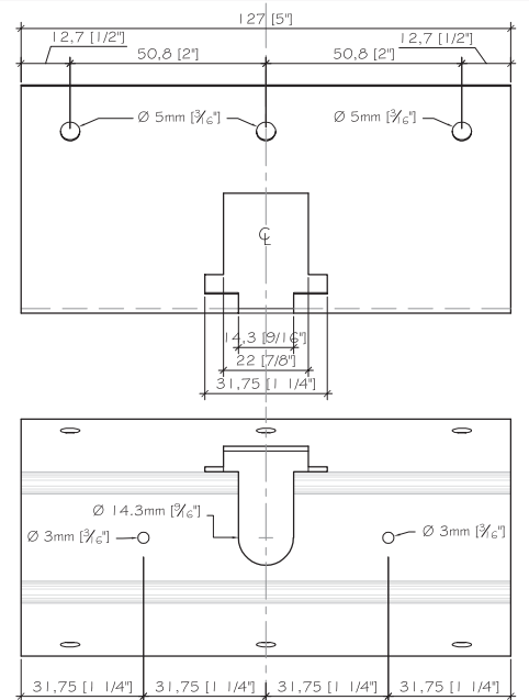
BRAK-IT No: 300 (1/4 - 5/16) PAT.PENDING
