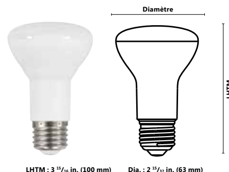
LHTM : 3 15/16 in. (100 mm) Dia. : 2 15/32 in. (63 mm)
