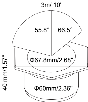
Max. Luminous intensity : 191 cd
