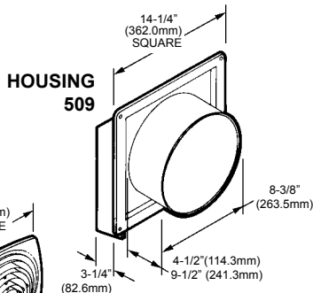
MODEL 509 GRILLE
