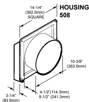
MODEL 508 GRILLE
