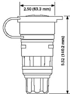
Dimensional Diagram
