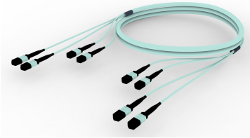
Ultra Low Loss (ULL) OM4 MPO12 (Pinned) to MPO12 (Pinned), Fiber Trunk Cable Assembly, 48-Fiber, Low Smoke Zero Halogen (LSZH)
