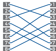
Cross-over Gigabit T568 B IEEE 802.3
